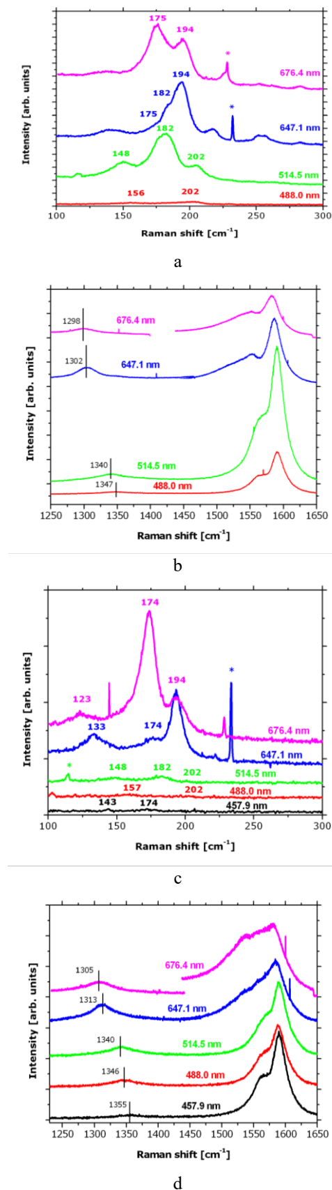
Fig. 3. Raman spectra of raw SWCNTs (a, b) and nitric acid-treated sample (c, d) for several laser excitation lines. See text for details.
